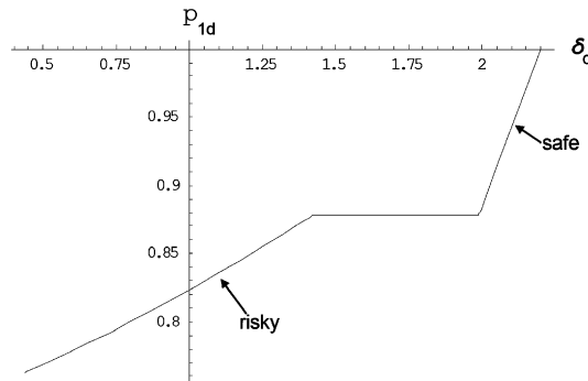
Fig. 4. The response of house prices to a change in outside demand \delta_d when \beta = 0.1 (and k = 0.4 and \sigma = 0.5 ). Borrowing is such that the risky agents default in period 2 for p_{1d} \leq 0.88 . This additional borrowing serves as a stabilizing force in the risky regime, and there is a financial decelerator in the transition from the safe to the risky regime.
