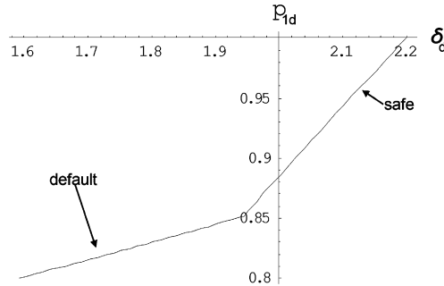
Fig. 3. The response of house prices to a change in outside demand \delta_d when \beta = 0.4 (and k = 0.4 and \sigma = 0.5 ). The equilibrium shifts from the safe regime to the default regime at p_{1d} = 0.85 . The safe regime is characterized by a financial accelerator, but strategic default serves as a stabilizing force in the default regime.
