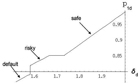
Fig. 5. The response of house prices to a change in outside demand \delta_d when \beta = 0.15 (and k = 0.4 and \sigma = 0.1 ). The equilibrium shifts from the safe regime to the risky regime at p_{1d} = 0.85 and then to the default regime at p_{1d} = 0.79 .
