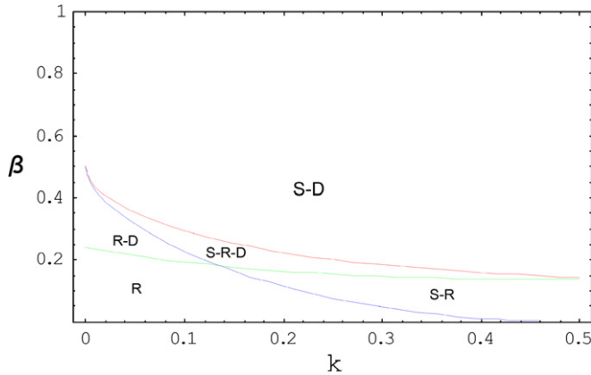
Fig. 2. The equilibrium regimes obtained as p_{1d} varies, for selected values of the bad types' default cost k and the measure of bad types \beta .
